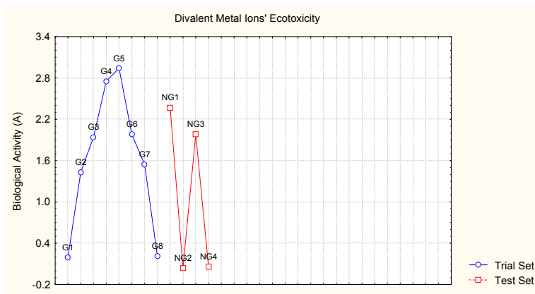
Figure 1. The plot of the divalent metal ions' EC 50 toxicities of Table I
